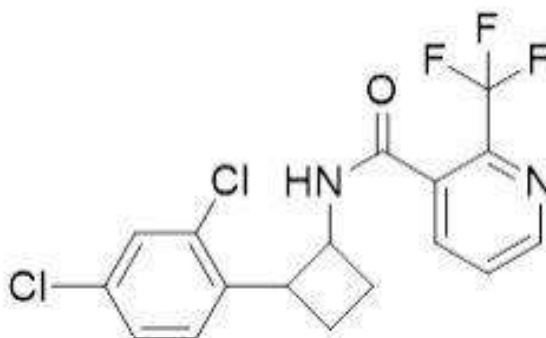
(A-1; ciclobutrifluram)
